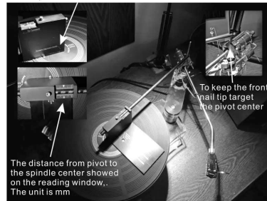
Placing the tonearm alignment hole to the spindle center
