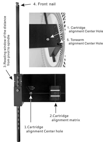
Placing the tonearm alignment hole to the spindle center
